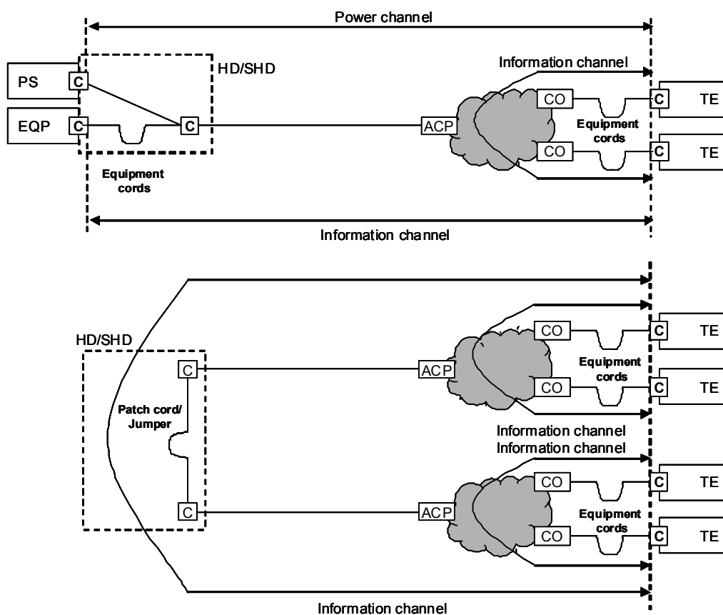
Figure 14 – Reference implementations for CCCB channels with HD or SHD
