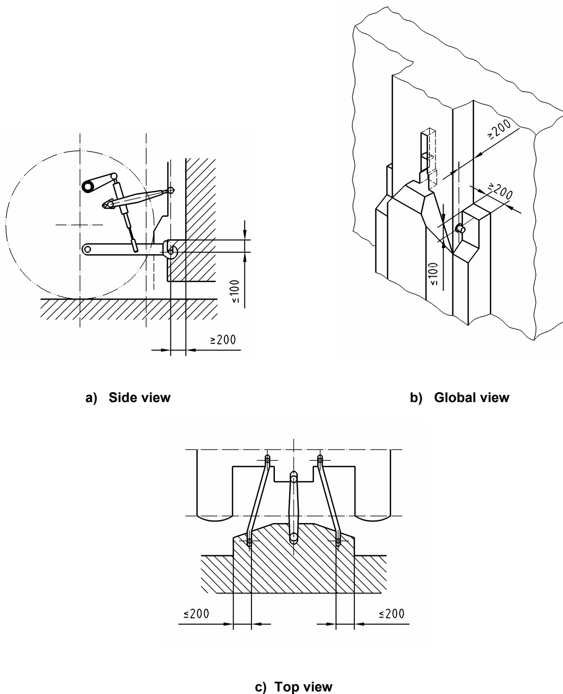
Figure 2 — Clearance zone
