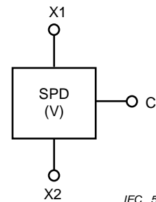
Figure 1c – Three-terminal SPD
