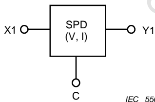
Figure 1b – Three-terminal SPD
