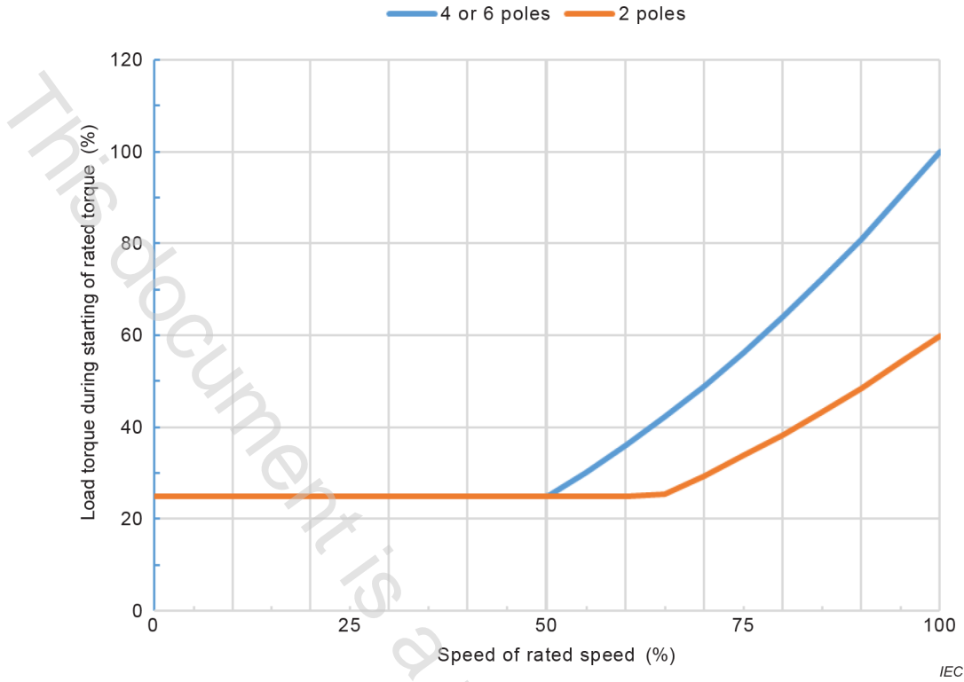
Figure 1 – Envelope of the load torque during starting: Load torque during starting in % of rated torque over speed in % of rated speed
