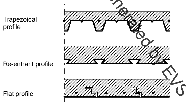
Figure 1.1 Typical examples of concrete slabs with profiled steel sheets with or without reinforcing bars
