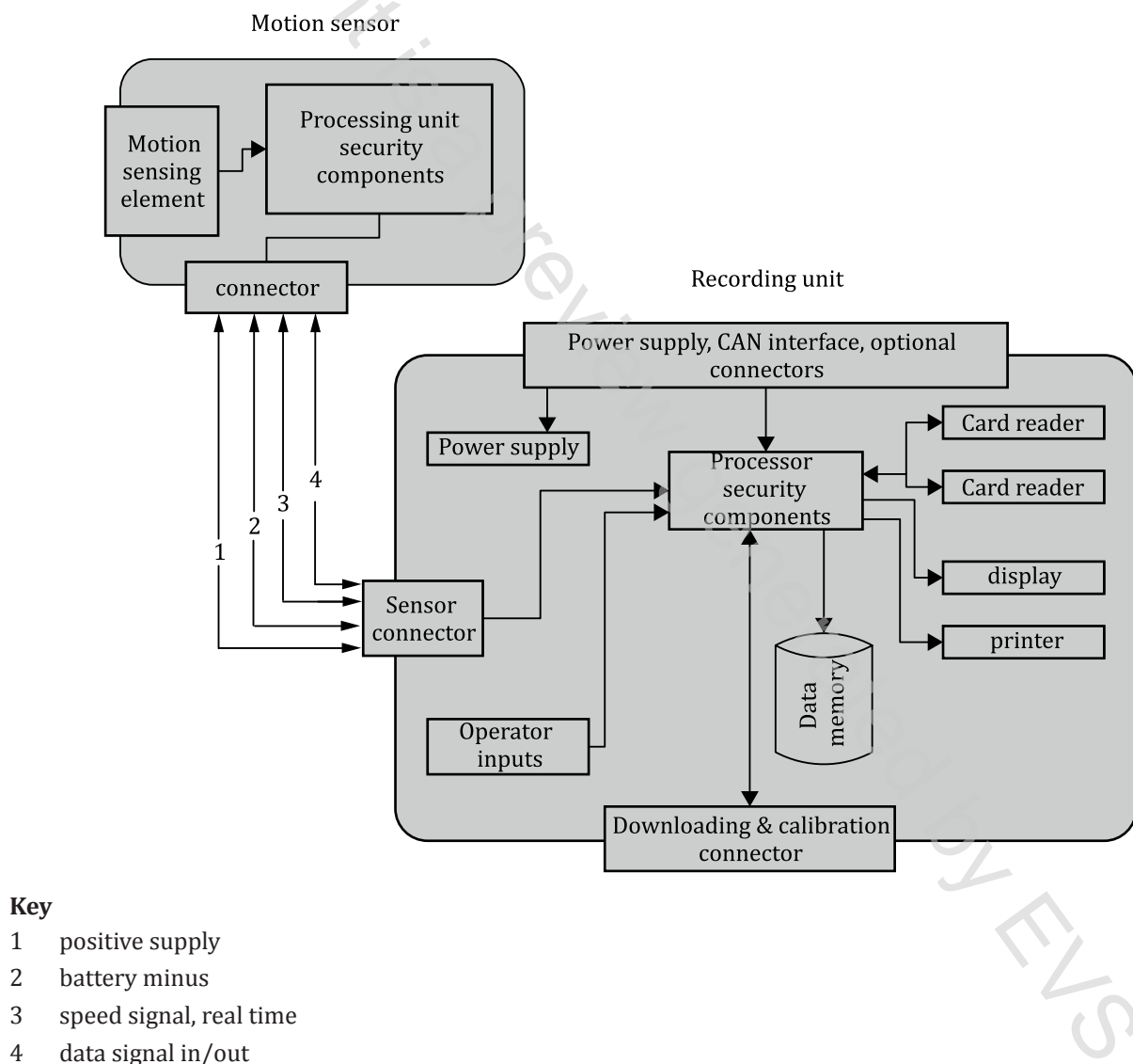
Figure 1 — Typical tachograph system
