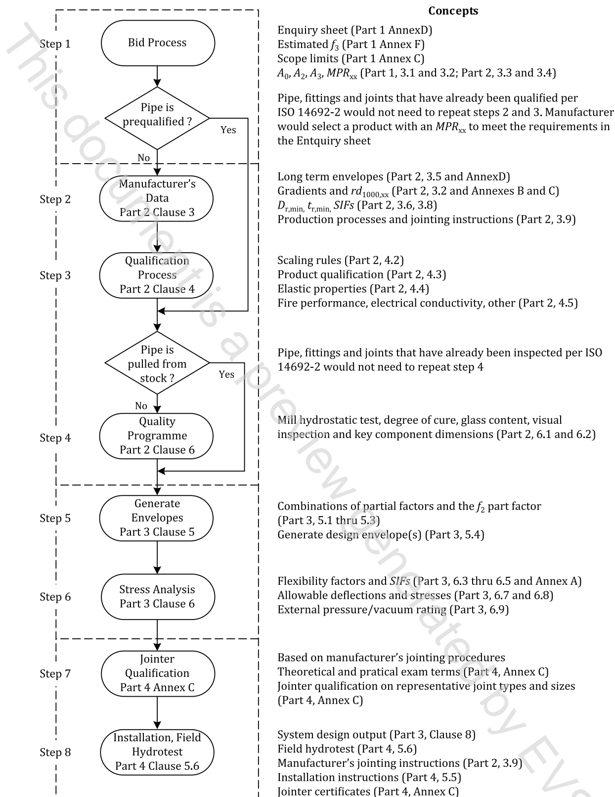
Figure 1 — Guidance on the use of ISO 14692 (all parts)
