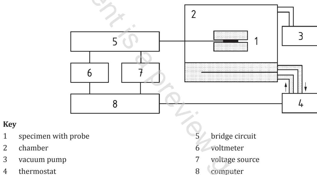
Figure 1 — Basic layout of the apparatus
