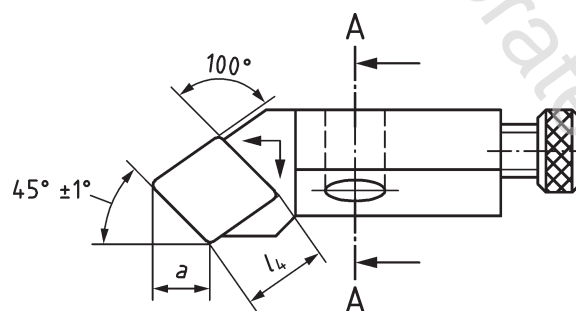
Figure 1 — Style S with height h_1 = 6 mm and 8 mm with rhombic indexable insert
