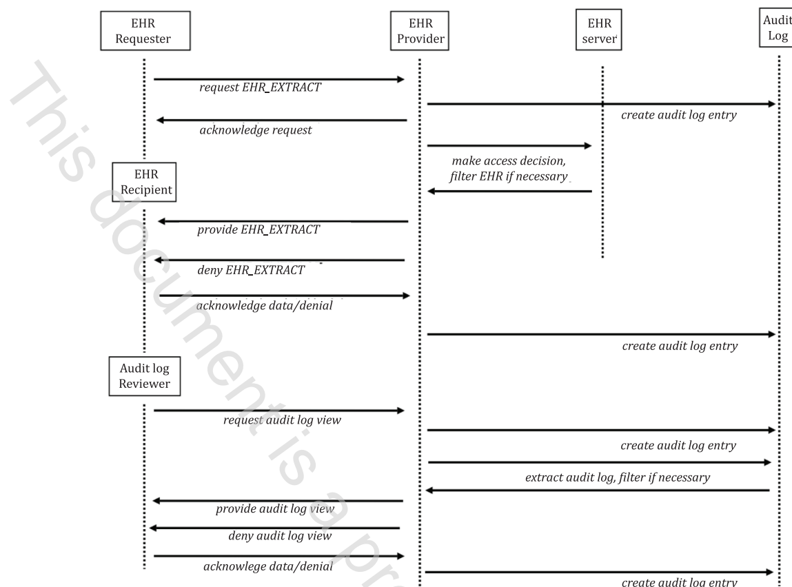
Figure 1 — Principal data flows and security-related business processes covered by this document
