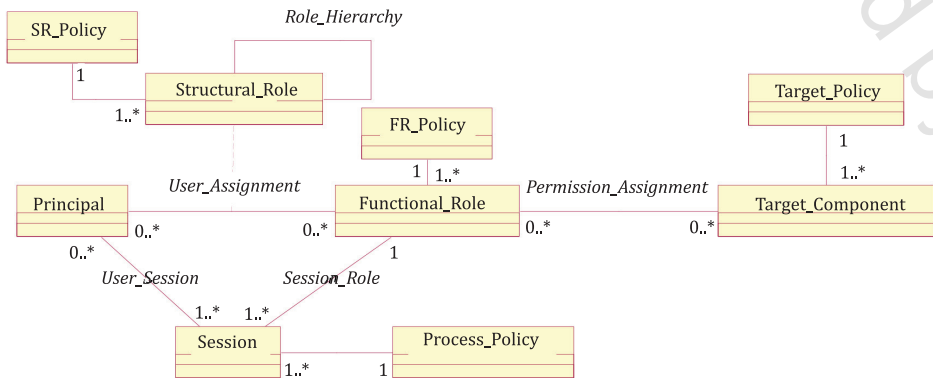
Figure 3 — Policy-driven RBAC Schema
