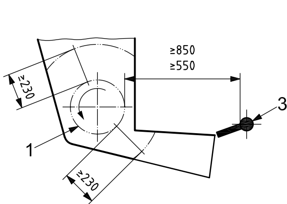
b) Side guarding
