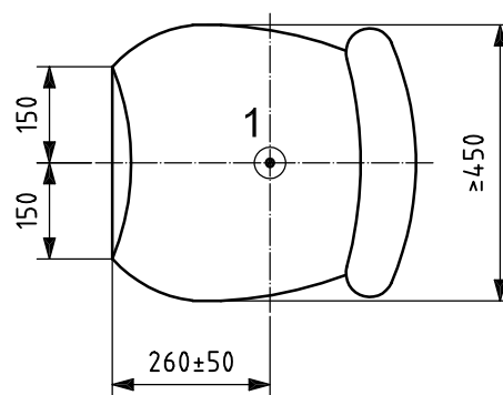
a) Intermediate seat adjustment
