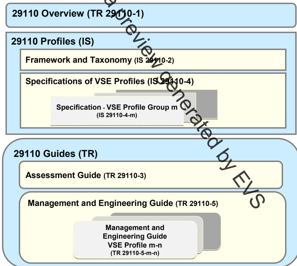
Figure 1 — ISO/IEC 29110 series
